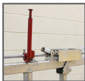
LEFT: EASY TAP / RELEASE PADDLES ON THE TOP OF THE HEADLOCK. ALSO SHOWN IS THE ANTI-TAMPER GUARD COVERING THE LOCKING MECHANISMS. RIGHT: SIMPLE AND HIGHLY VISIBLE RED HANDLE SIGNALS A LOCKED SECTION.
